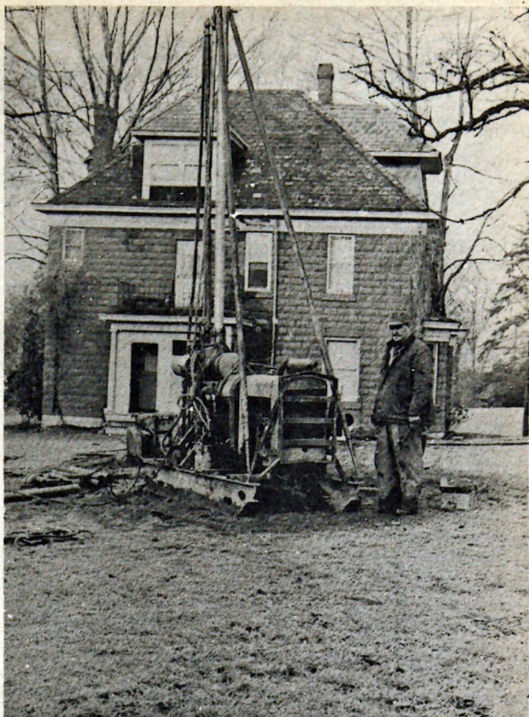
DRILLING ONE HOLE A DAY , the Pennsylvania Drilling Company will take 25 test borings to determine amount and depth of rock, clay and sand on the site of the new library. This information enables contractors to submit a more accurate bid, and structural engineers will have a better estimate of the amount of foundation necessary.
