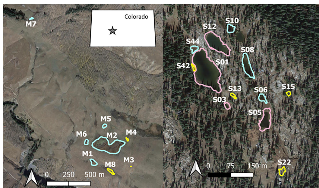
Fig 2. The southwest corner of the montane site (left) is located at 38°56' 31" N, 106°58'46" W and the southwest corner of the subalpine site (right) is located at 39°01' 39" N, 107°03'53" W. Permanent ponds are in red, semi-permanent in blue, and temporary in yellow.
