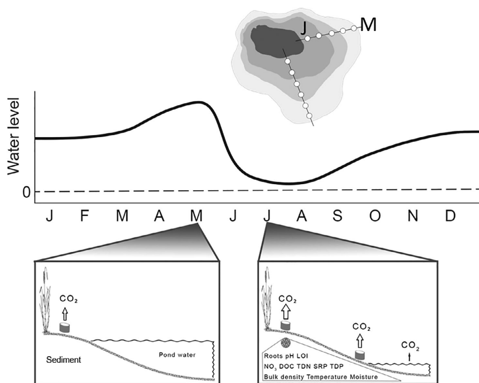
Fig 1. A conceptual hydrograph for these snowmelt driven ponds shows melt-out in spring. Ponds then steadily dry down over the course of the season until they refill with snow in late fall. As ponds dry down, they expose margins of sediment from which we collected estimates of CO 2 flux. Upper figure conceptual overview of a pond shows how pond margins might shrink over time from May (M) to July (J) and how transects were oriented toward the deepest part of the pond (gauged by the shrinking pond margins) with collars placed progressively as the pond water area shrunk. We considered direct effects of hydrology (exposure date and associated temperature and moisture) as well as how overall hydrologic patterns could affect sediment characteristics which might then influence CO 2 flux.
