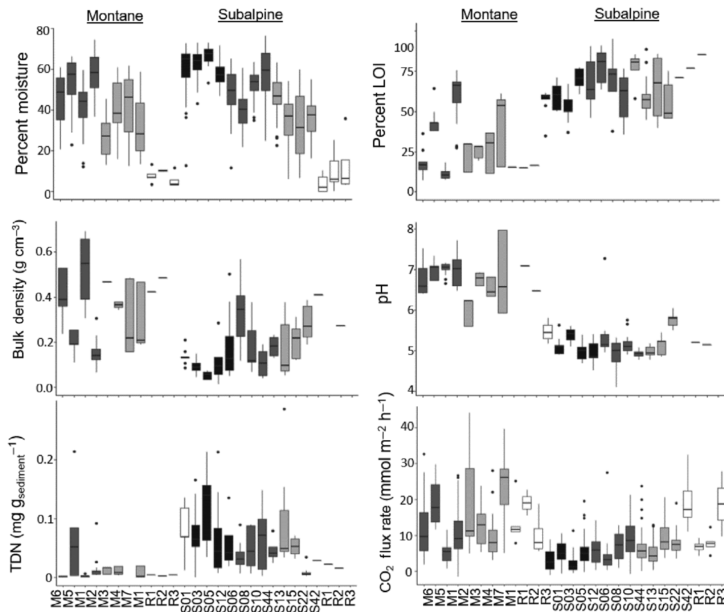
Fig 3. Boxplots of all collar measurements from each pond (line represents median, boxes represent interquartile range, dots represent outliers). Dark fills are permanent ponds; medium fills are semi-permanent ponds, light points are temporary ponds, and white fills or single measurements are reference sites. Additional data are shown in Supporting Information Fig. 3, and summary statistics are reported in Table 1. Flux rate refers to CO 2 flux rate.
