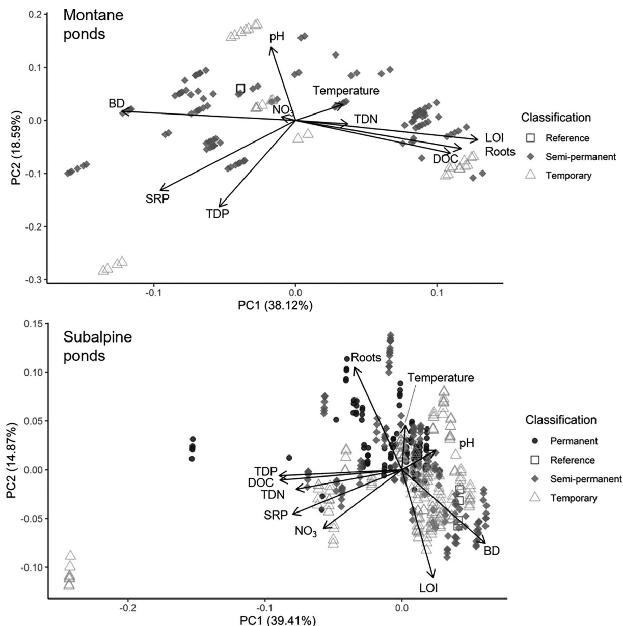
Fig 4. A PCA of pond sediment properties at each site was used to reduce dimensions of variance and test for the effects of pond hydroperiod classifications and sites. Data points are soil characteristics within each collar.
